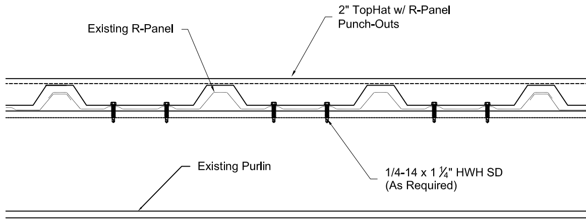
No Deflection Limiters - Field Zone As Determined by Engineering
