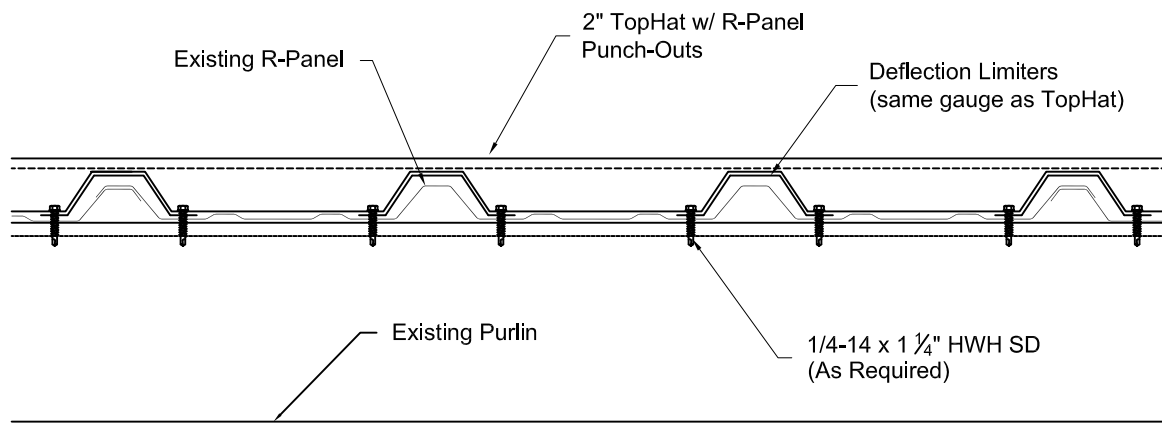
Deflection Limiters - Edge and Corner Zones (if required) As Determined by Engineering
