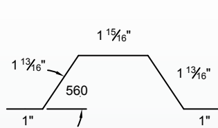
R-Panel Profile
